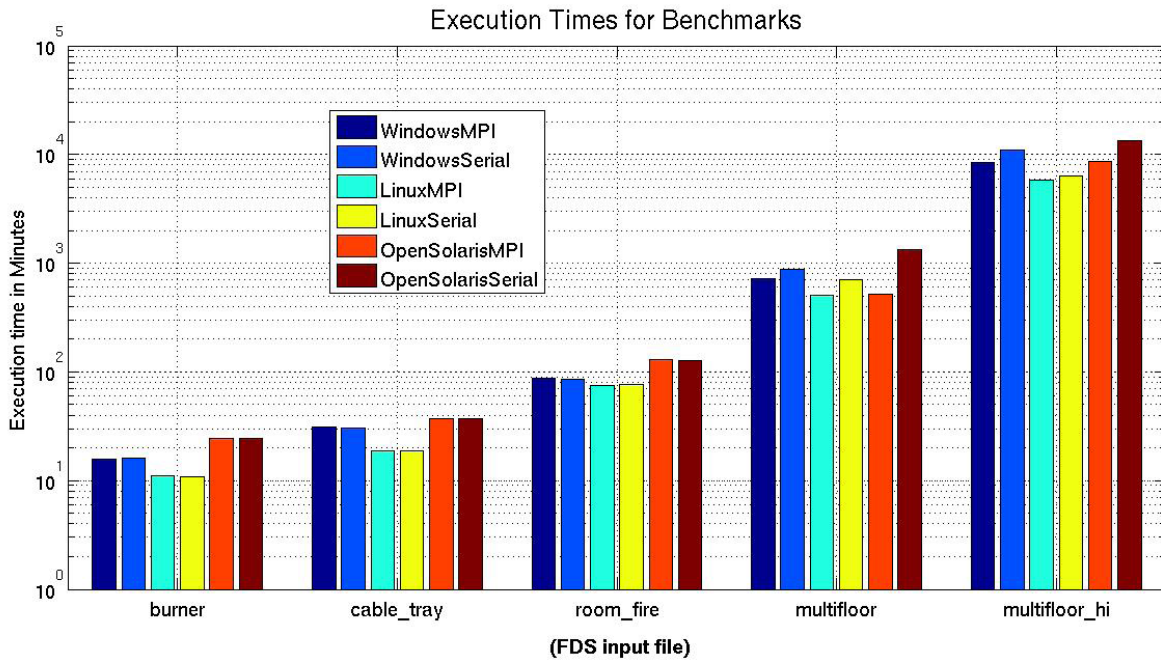
Figure 1.- Execution benchmark times for small scale systems
