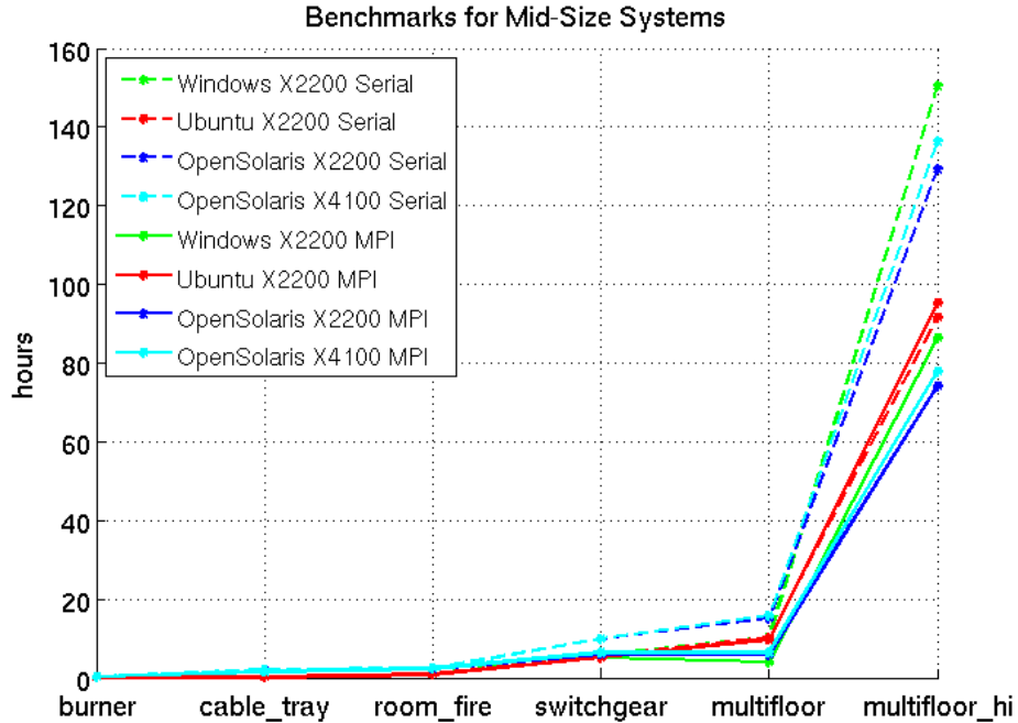
Figure 2- Execution benchmark times for mid-scale systems
