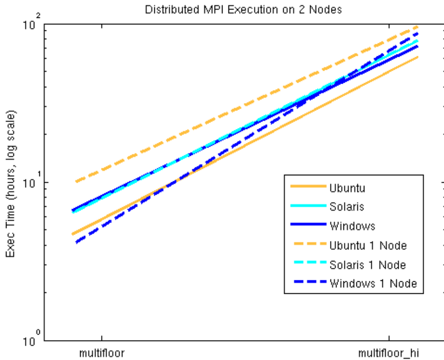
Figure 3- Execution benchmark times for large-scale systems
